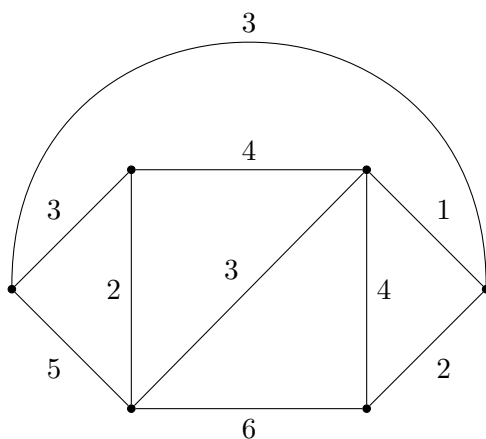
Figure 4.7: Is there a Hamiltonian cycle with weight 15?
