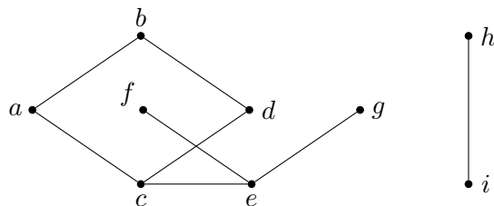
Figure 4.4: An example of a graph with 9 vertices and 8 edges.
