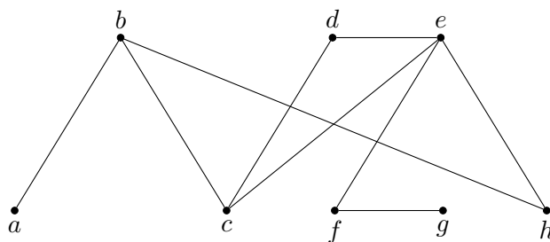
Figure 4.5: A graph with 3 cycles: bhecb , cdec , and bcdehb .
