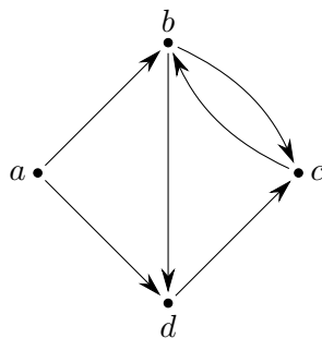
Figure 4.1: A 4-node directed graph with 6 edges.
