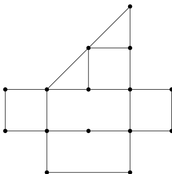
Figure 4.6: Is there a walk that includes every edge exactly once?
