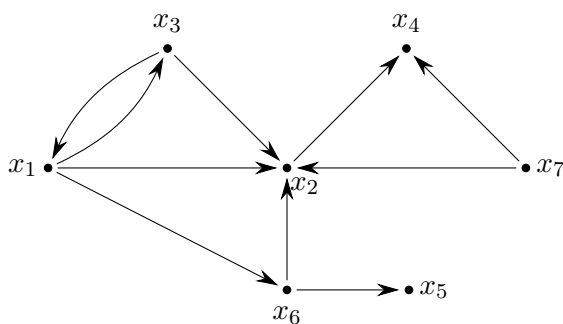
Figure 4.3: Links among Web Pages.
